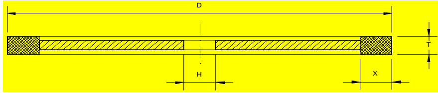
6" Diameter 1 - 1/4" Bore
